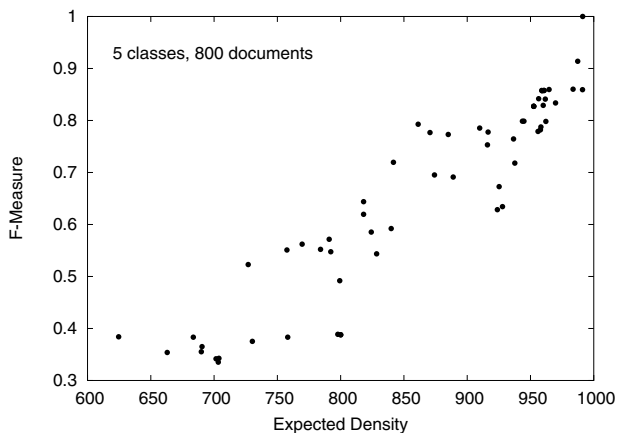
Figure 8. Correlation of the F -Measure and the \bar{\rho} -Measure for genuine clusterings.
